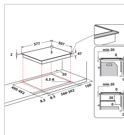
CTAR 7642 IN
